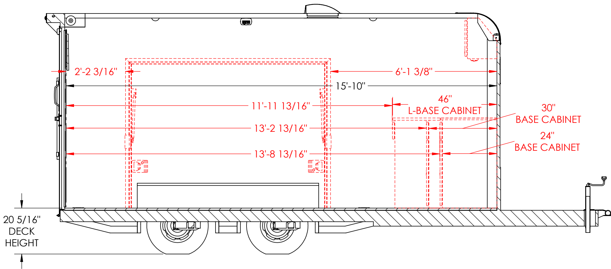
INTERIOR ROAD SIDE SECTION A-A
